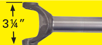
Part# FTSFS002
